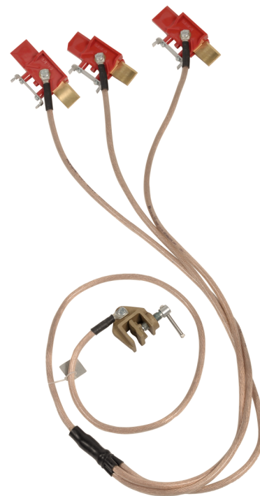
THREE-PHASE SHORT-CIRCUITING DEVICE
